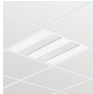
FLEXBLEND RECESSED, module 600 - 840 neutral white - Power supply unit regulating external - Push-in connector and pull relief
